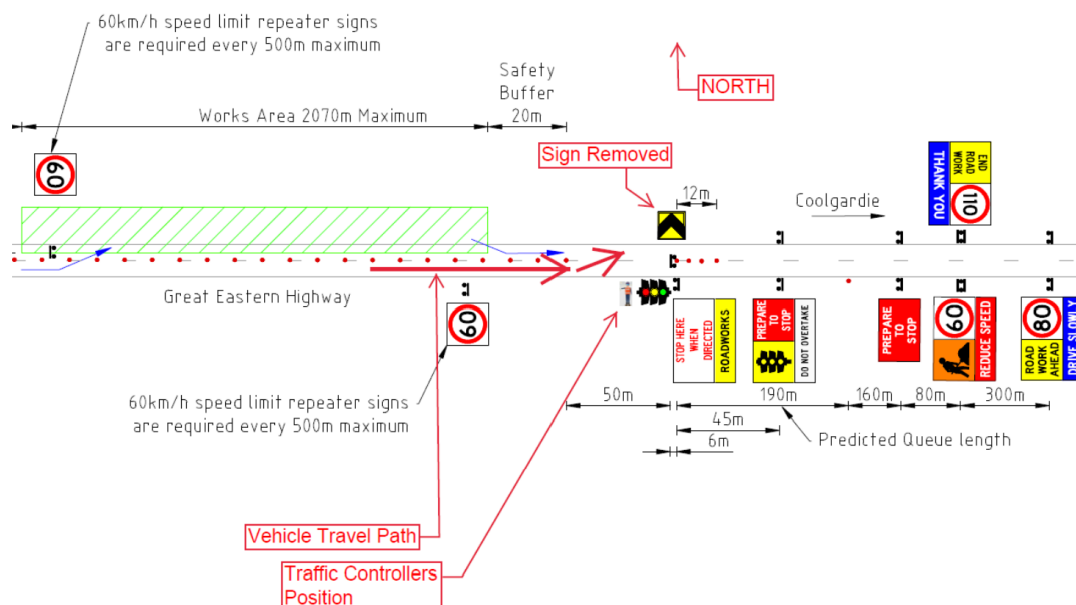
Diagram of the TM setup and incident
